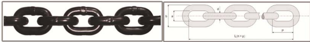
G80 Lifting Chain-G80起重链
